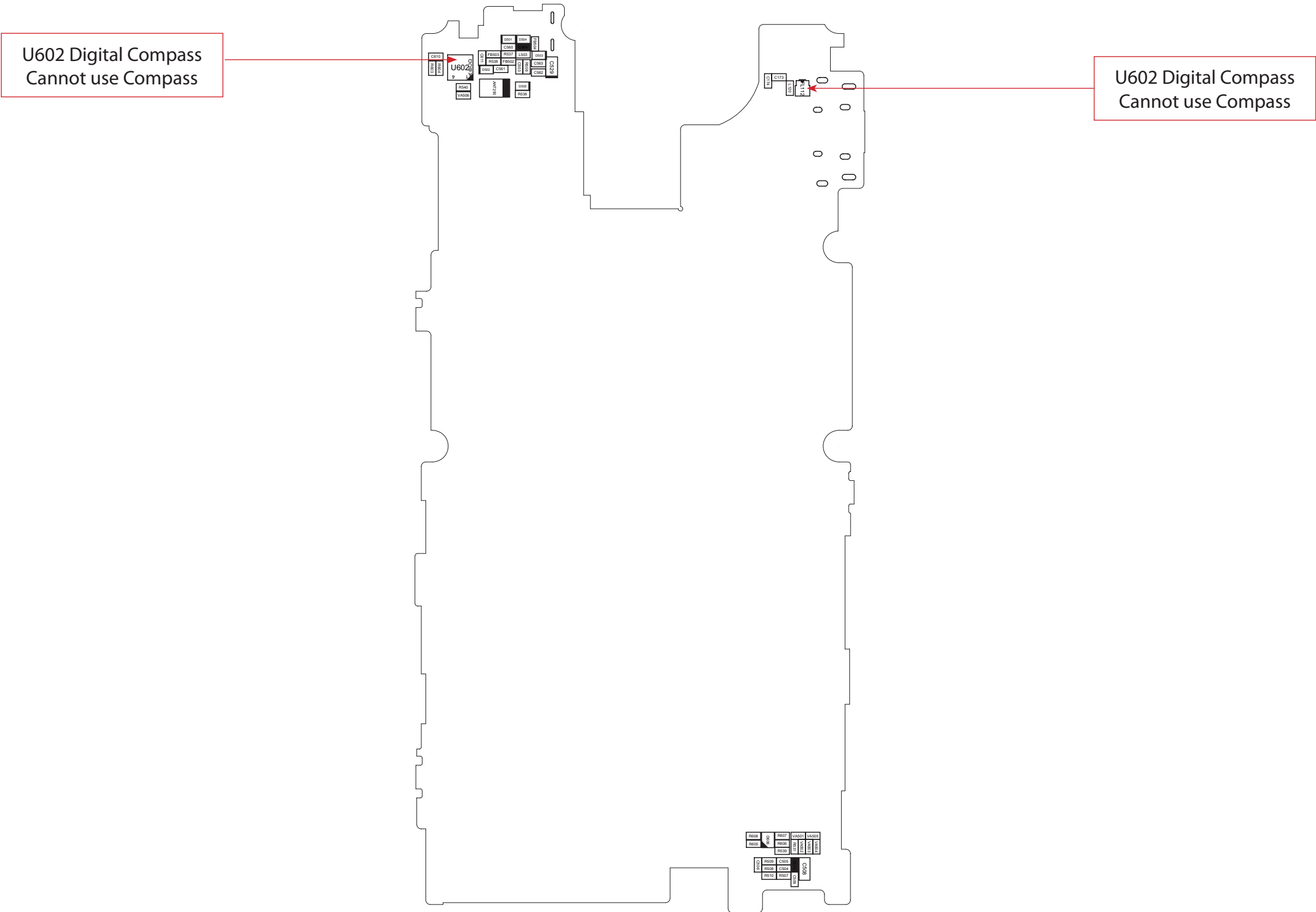
GT540_MAIN_SPFY0221301-1.0_TOP
