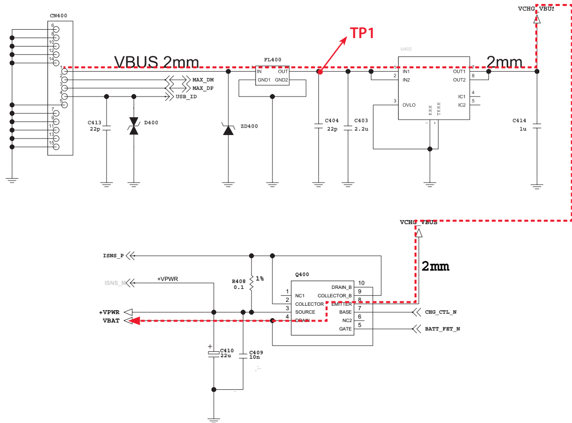
Figure. Charging Current Flow
