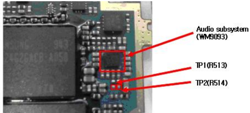
TP1(R513), TP2(R514)
