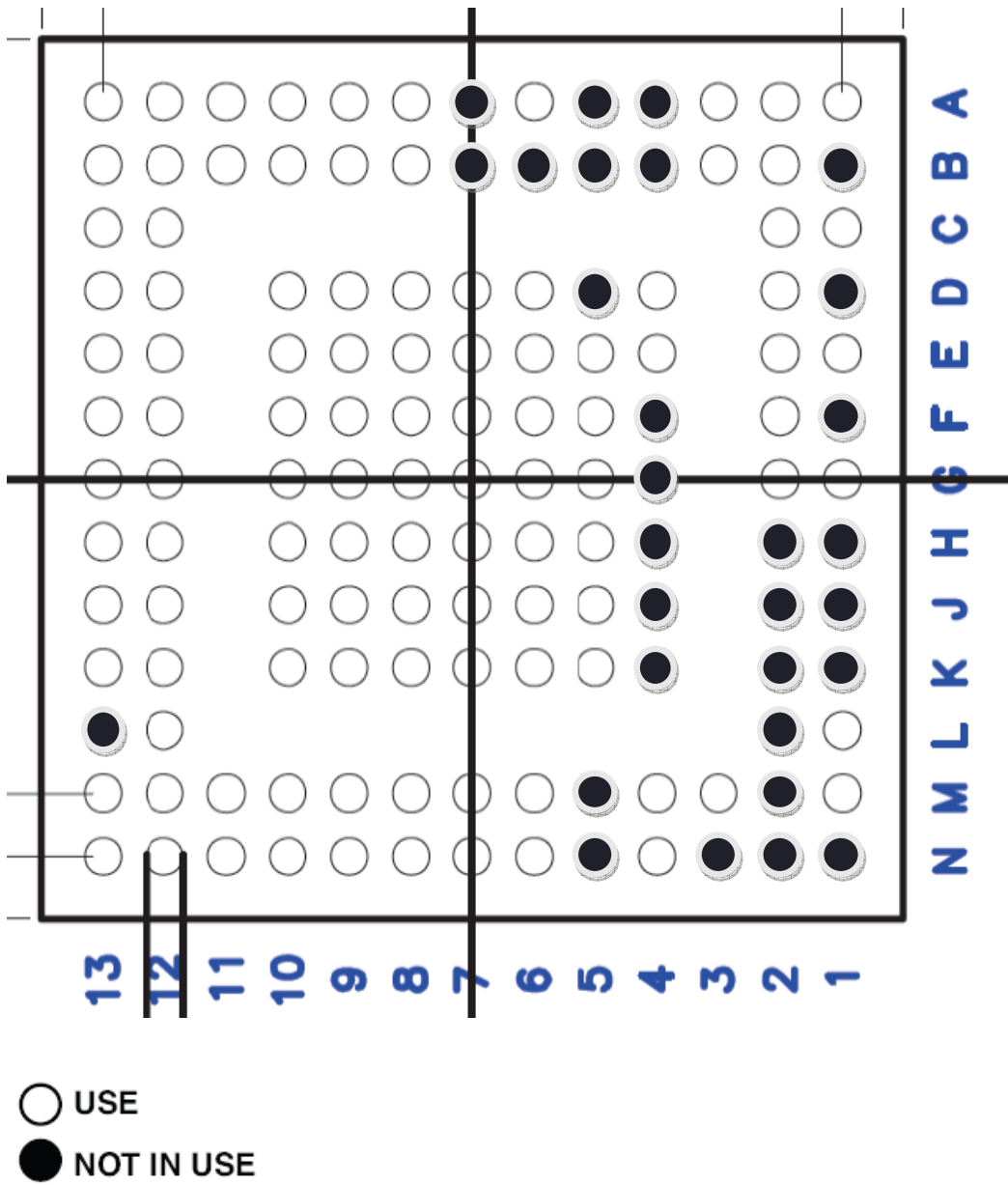
PM7540(PMIC)
