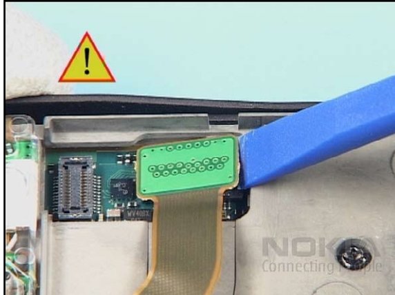
20. Carefully open the UI MODULE connector taking special care to the surrounding components.
