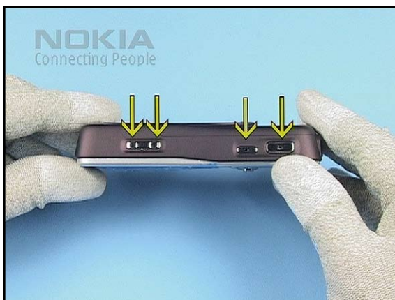
46. Finally, check the functionality of the keys and ensure that there are no gaps between the covers.
