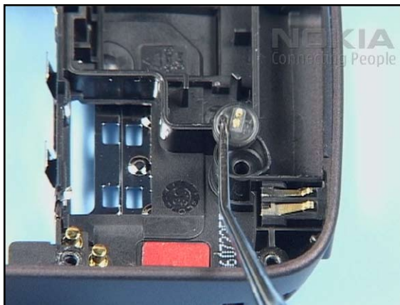
44. Remove the MICROPHONE with the dental pick.
