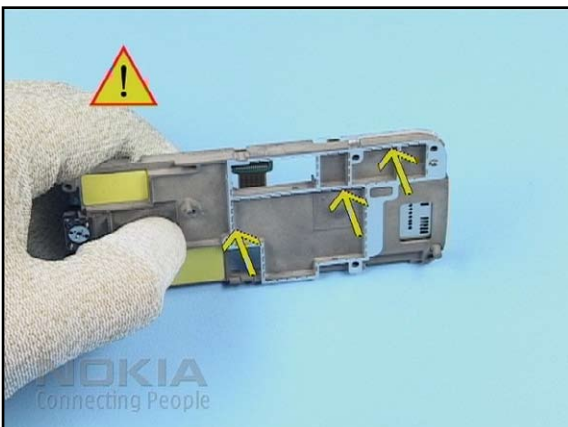
29. Take special care to the BASEBAND GASKET.
